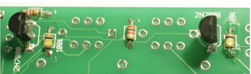
Above: 100k trimpot on far left edge Above: two 2N7000's on the top edge, left side
